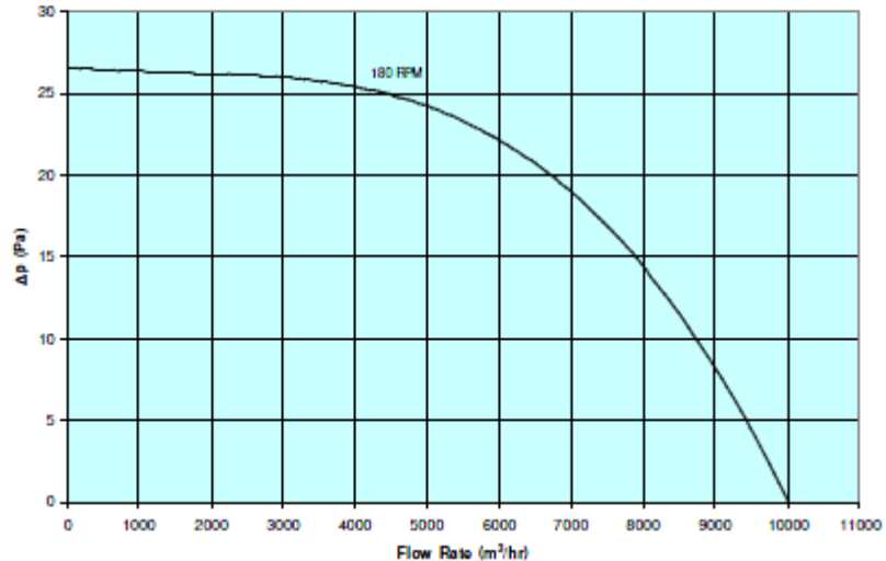
Performance Chart
