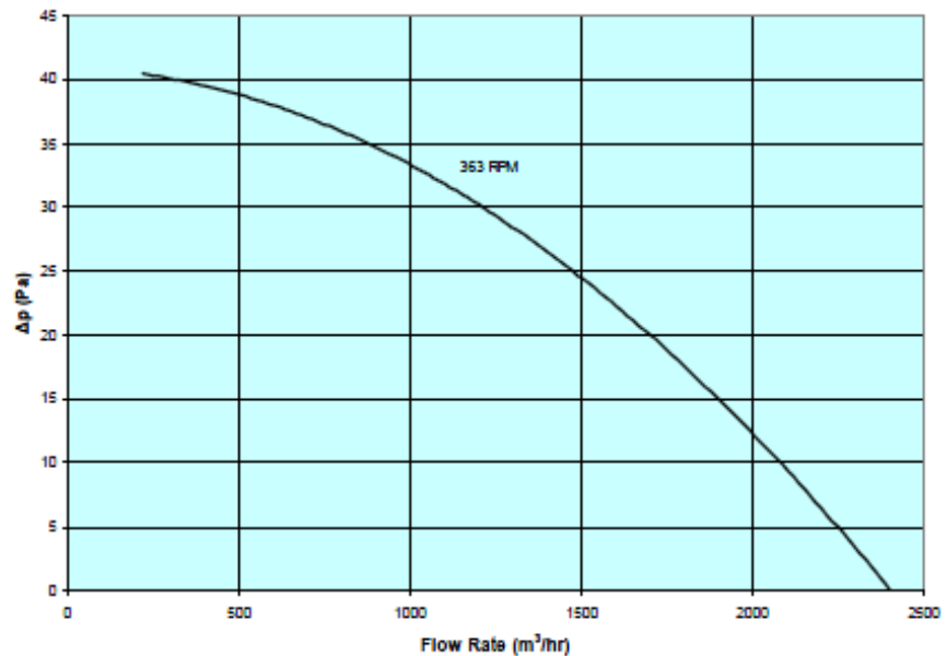
Performance Chart
