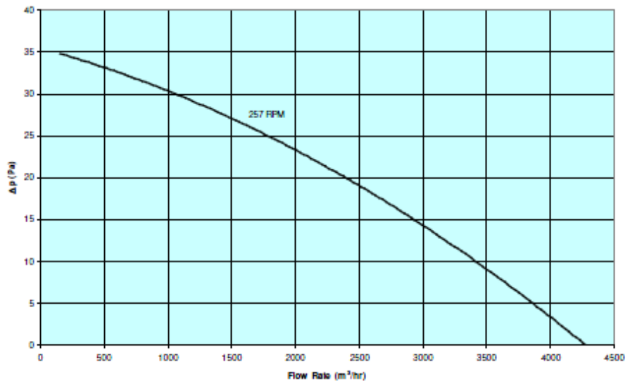
Performance Chart
