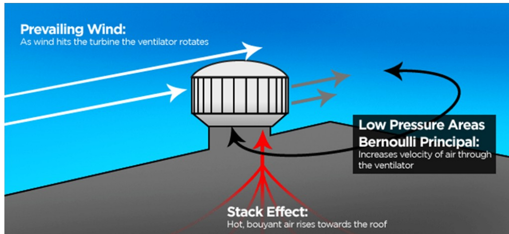
Figure 2: Air flow patterns for hybrid ventilator turbines.
