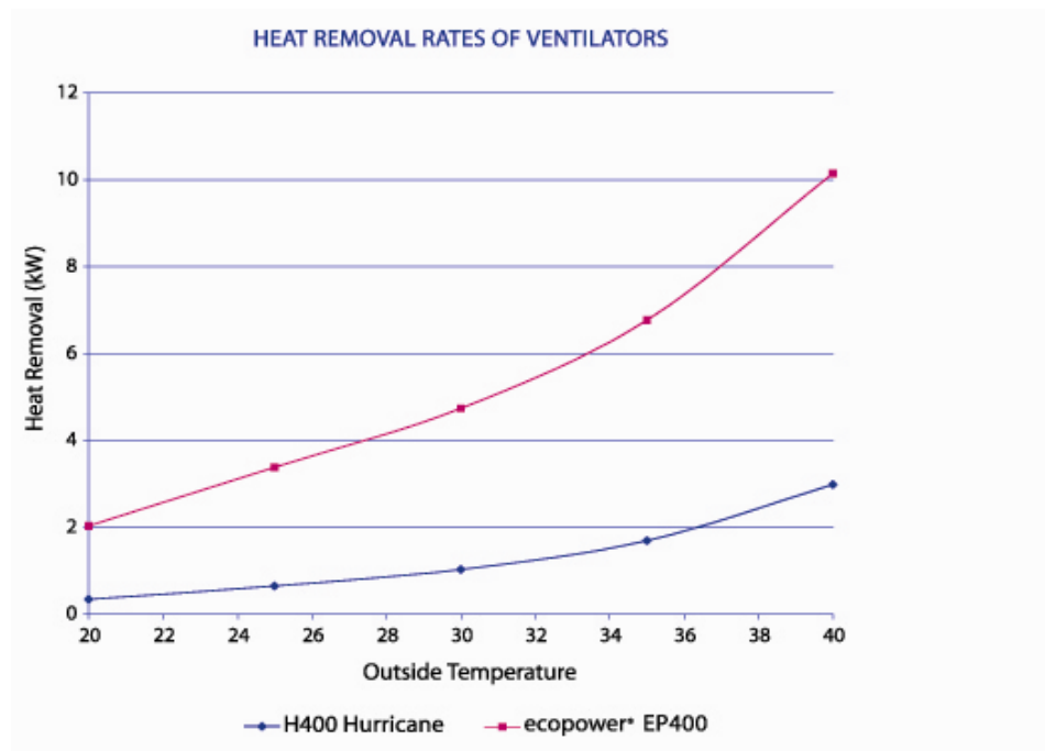
Figure 3: Heat removal rates of natural Edmonds Hurricane ventilators in comparison to powered ecopower units
